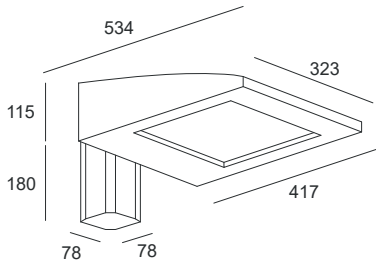
Cairo Street Light 3,50 Kg
