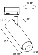
AVANA Track Spotlight Maxi
