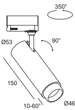
AVANA Track Spotlight
