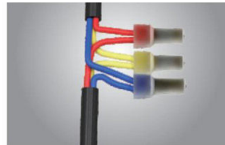
Exposed junction
