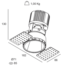
Flo Wall Washer recessed flush-fitting
