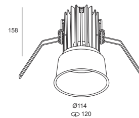
Flo recessed flush-fitting Maxi
