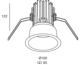
Flo Recessed Backlogged 0,45 Kg
