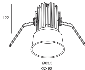
Flo recessed flush-fitting 0,45 Kg
