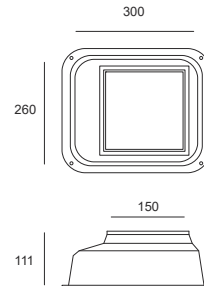
Cola maxi square recessed formwork
