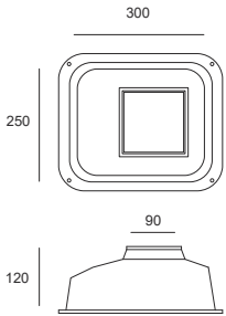
Cola square recessed formwork
